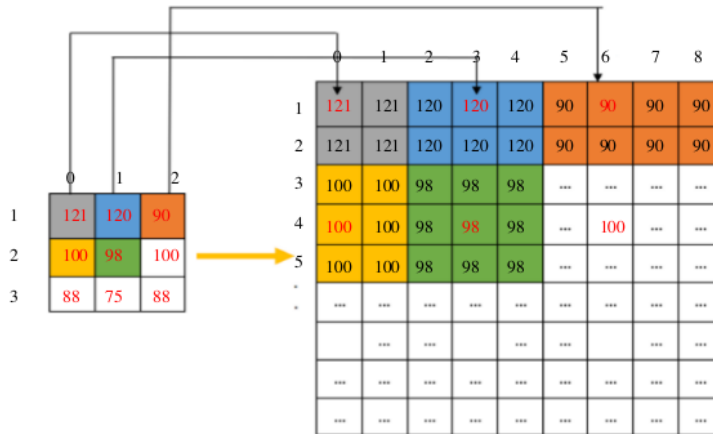
Fig. 8: Haar-like feature
