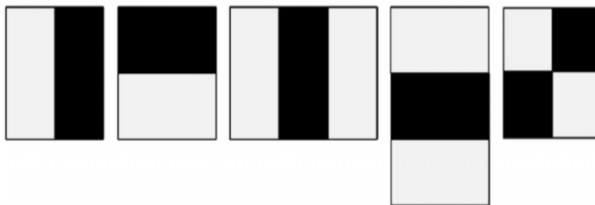
Fig. 4. Haar-like feature
